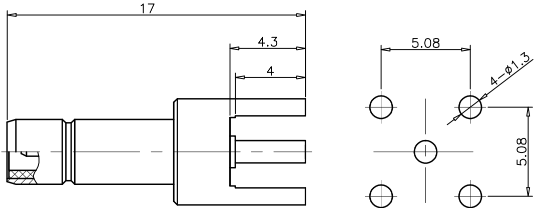
Mounting Detail
